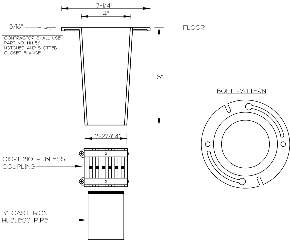
PART NO. NH 56 NOTCHED AND SLOTTED CLOSET FLANGE
