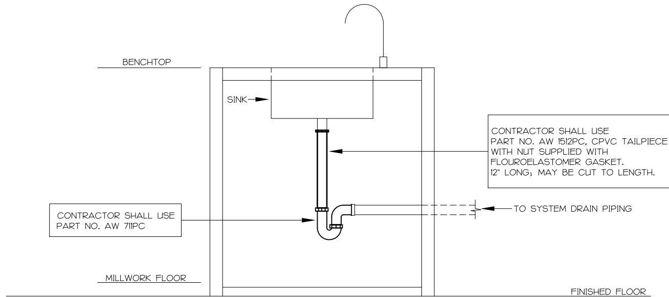
BENCH SINK L.A. PATTERN P-TRAP WITH UNION FITTING - SIDE ELEVATION
