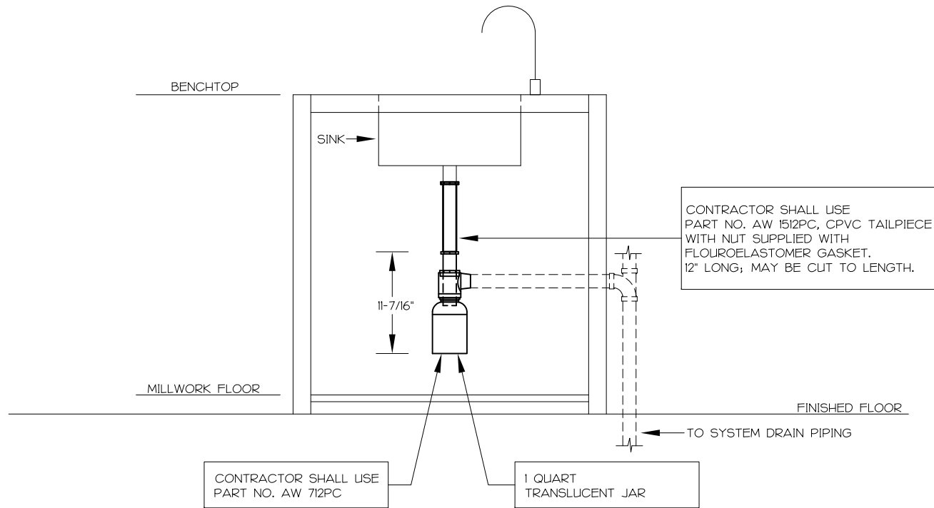
BENCH SINK JAR TRAP FITTING - SIDE ELEVATION
