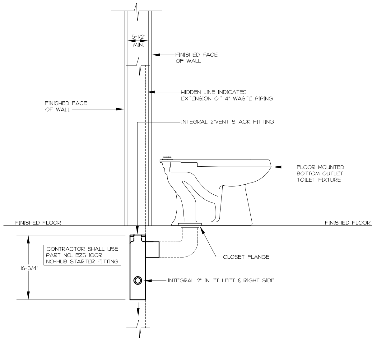
SINGLE FITTING RIGHT HAND UNDER-SLAB - LEFT SIDE ELEVATION
