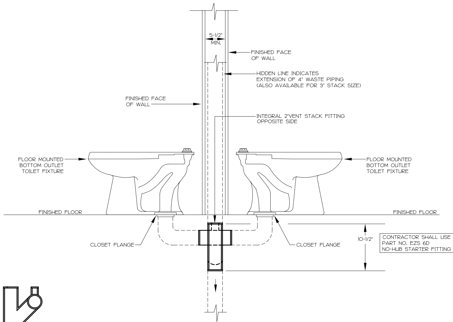
DOUBLE FITTING RIGHT HAND UNDER-SLAB - LEFT SIDE ELEVATION - VERTICAL CONFIGURATION
