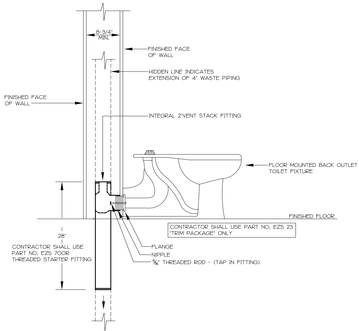
RIGHT HAND FITTING - LEFT SIDE ELEVATION
