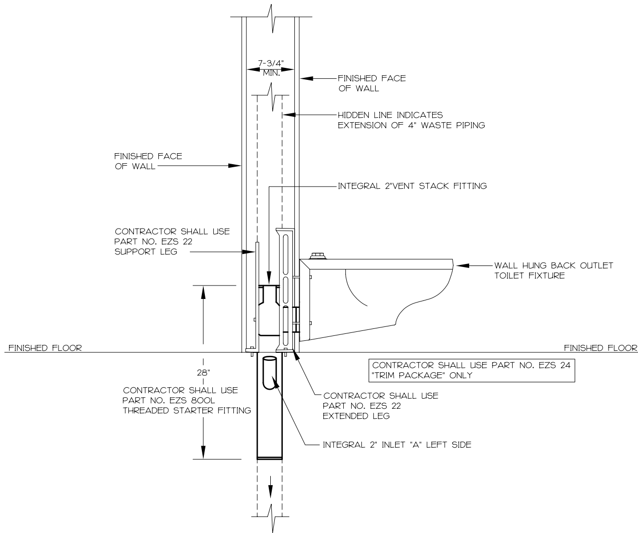
LEFT HAND FITTING - LEFT SIDE ELEVATION
