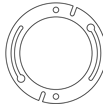
AVAILABLE BOLT PATTERN
