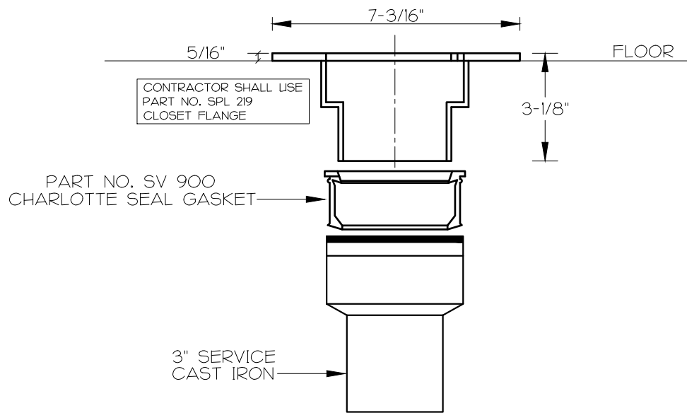
PART NO. SPL 219 GREENSBORO REDUCING CLOSET FLANGE
