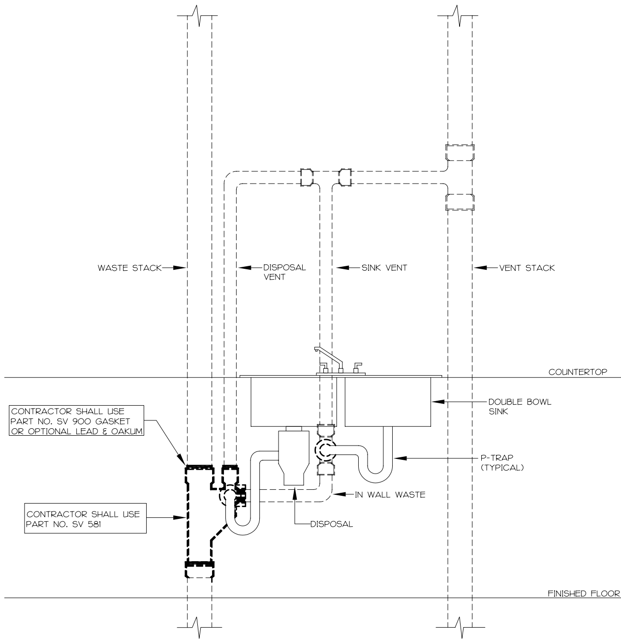
DOUBLE SINK STACK FITTING - FRONT ELEVATION
