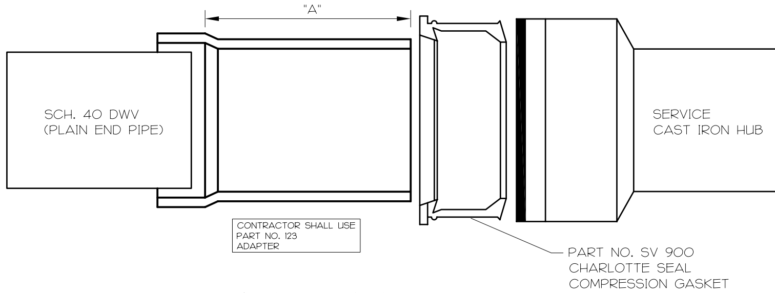
PART NO. 123 ADAPTER HUB x SPIGOT (ADAPTS DWV SPIGOT TO SV CAST IRON HUB)
